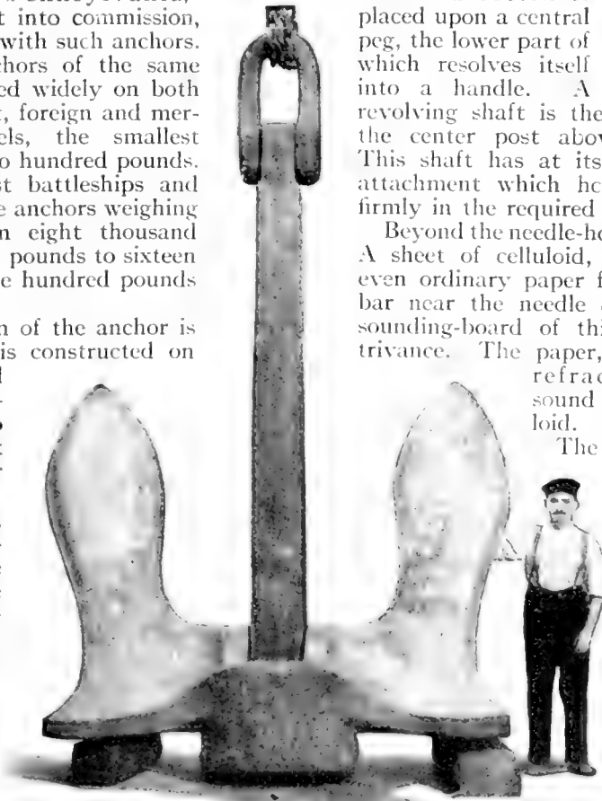
The Anchor Is Constructed on the Principle of a Ball and Socket, with the Fluke or Main Portion in One Piece
